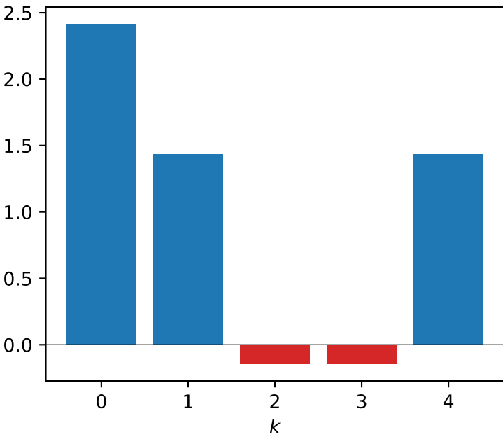
\mathbb{Z}_5 amplitude split (3+2)
