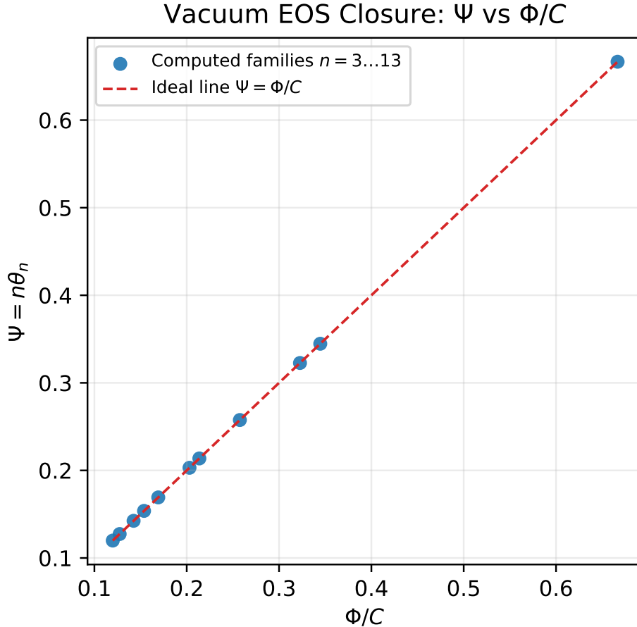
Figure 4: Archived Paper X vacuum equation-of-state check: the equilibrium variable \Psi_s tracks \Phi/C across the torus-knot family. In this synthesis paper the same relation is used only as a bridge assumption for cosmological hypotheses, not as direct evidence for the dark sector.
