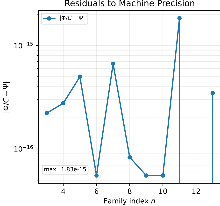
Figure 5: Archived Paper X residual panel. Residuals near numerical precision support internal consistency of the vacuum equation-of-state calculation; external cosmological validation remains a separate requirement.
