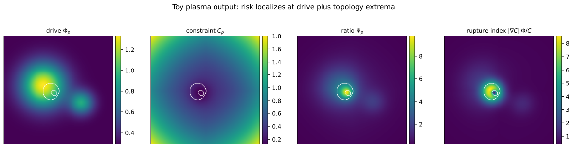
Figure 4: Generated plasma output. The rupture index combines drive, constraint, and constraint-gradient information. In the toy field, risk does not follow the drive field alone. Summary table: table5_plasma_rupture_index_summary.csv .
