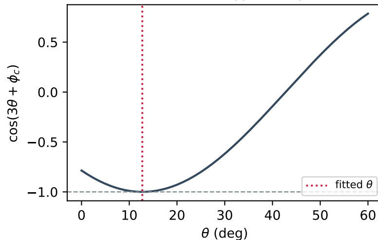
(b) Chiral energy surrogate
