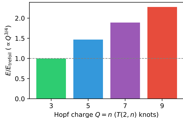
(a) Faddeev–Niemi scaling
