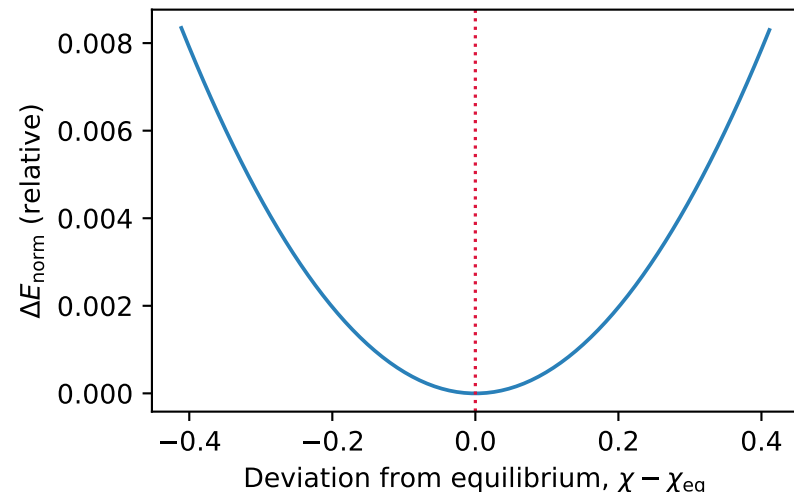
(c) E_{\text{norm}} near equilibrium
