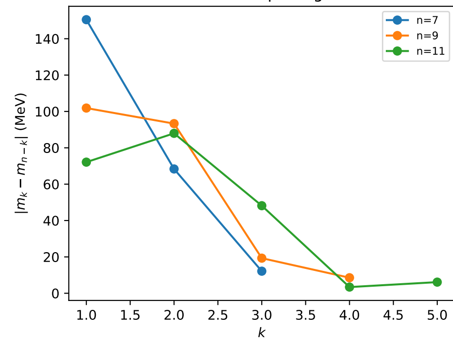
Doublet splittings
