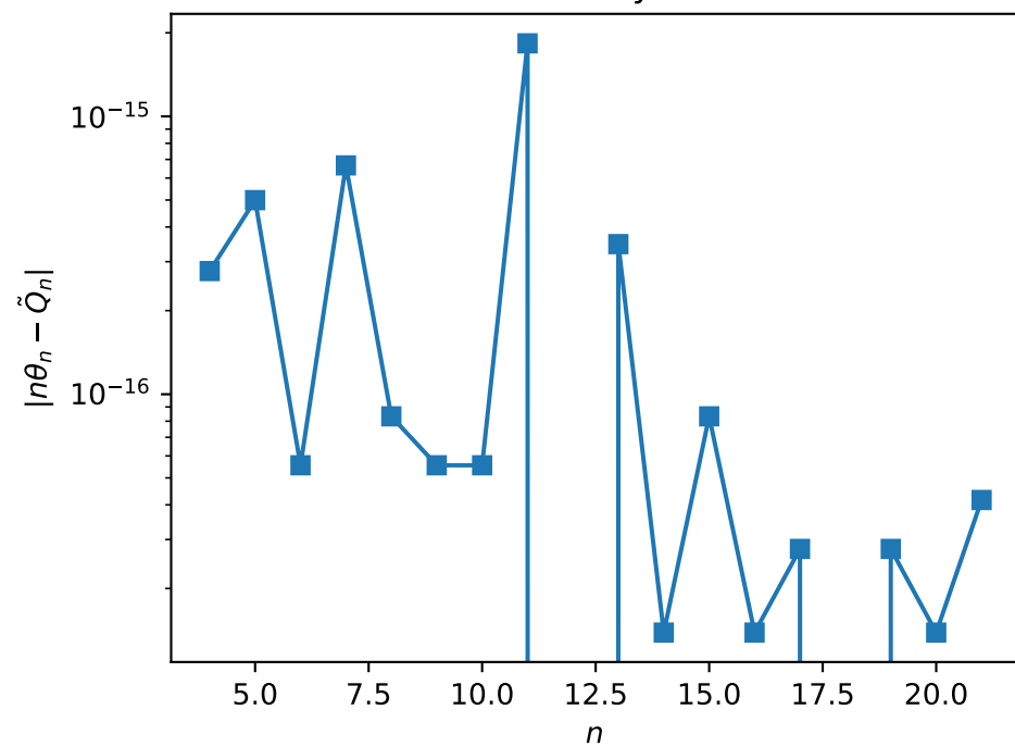
Self-consistency residuals
