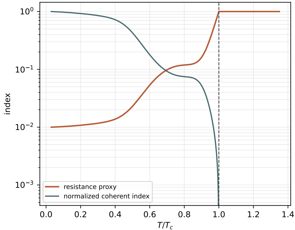
Dissipation collapse with retained phase constraint
