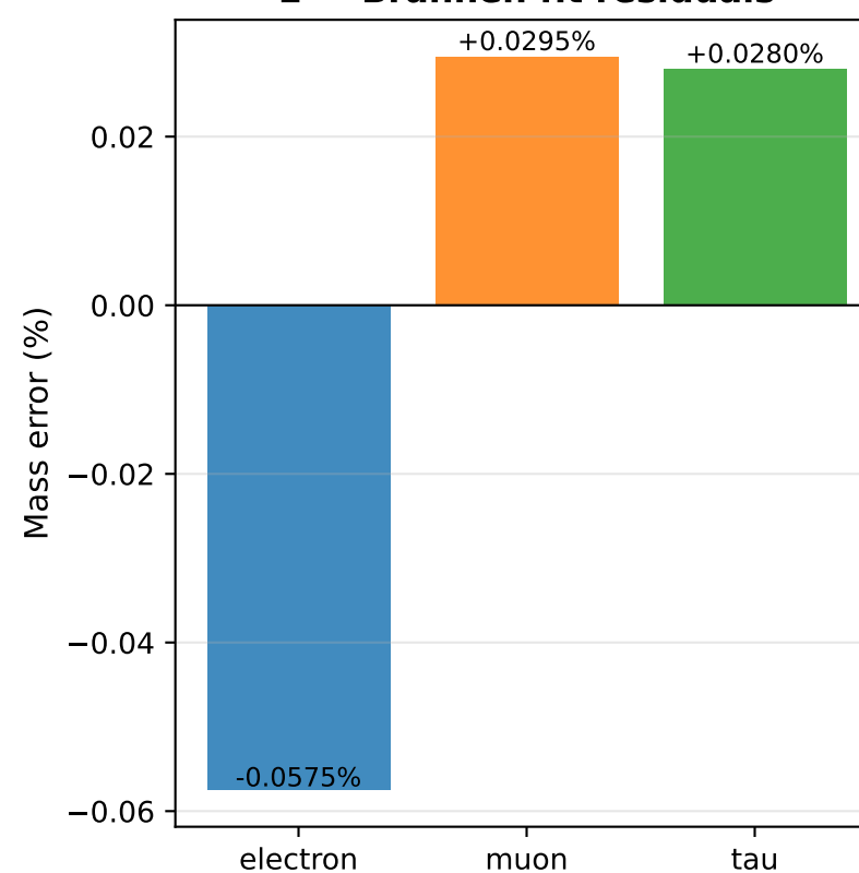
E — Brannen fit residuals
