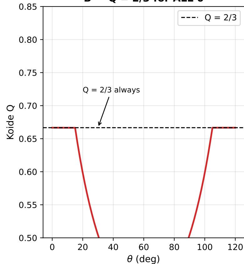
B — Q = 2/3 for ALL \theta
