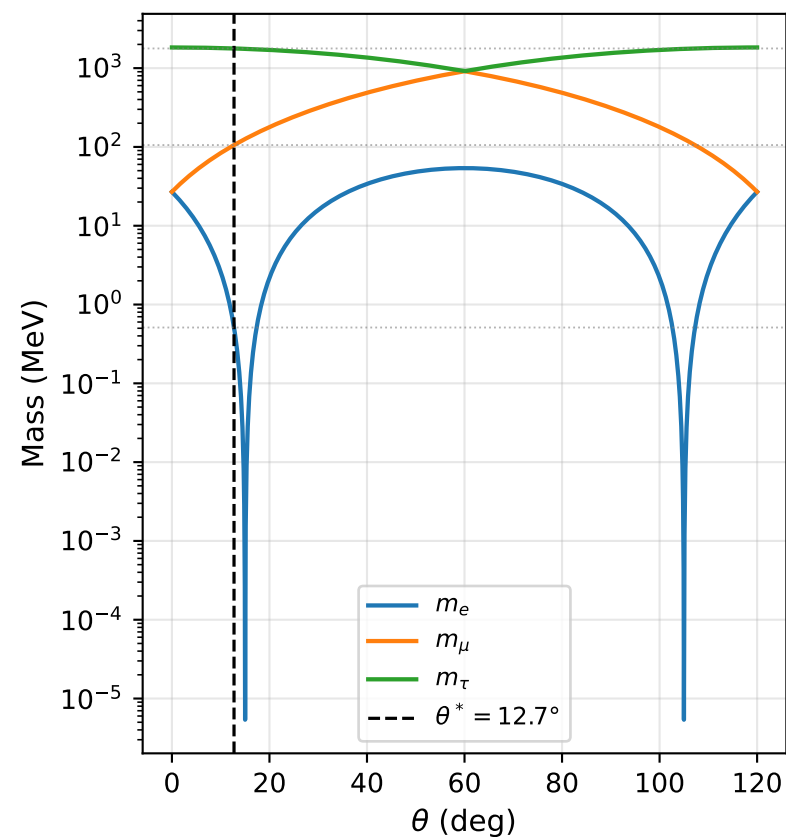
A — Brannen masses vs \theta
