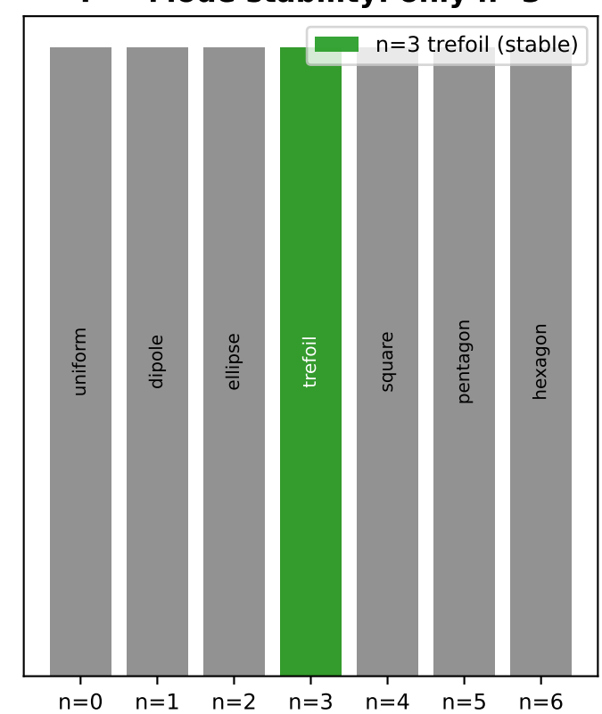
F — Mode stability: only n=3
