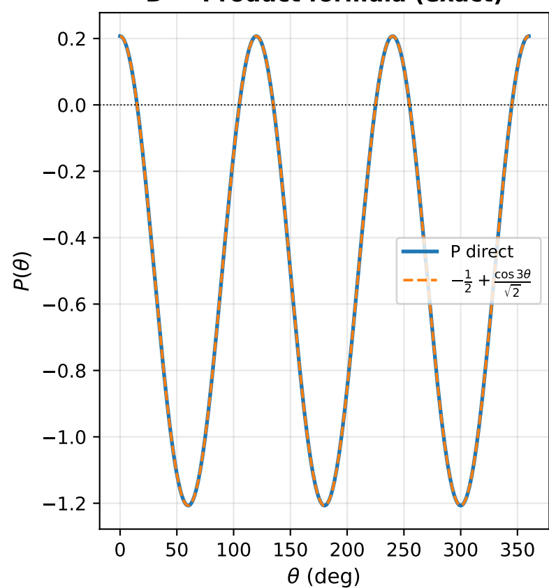
D — Product formula (exact)
