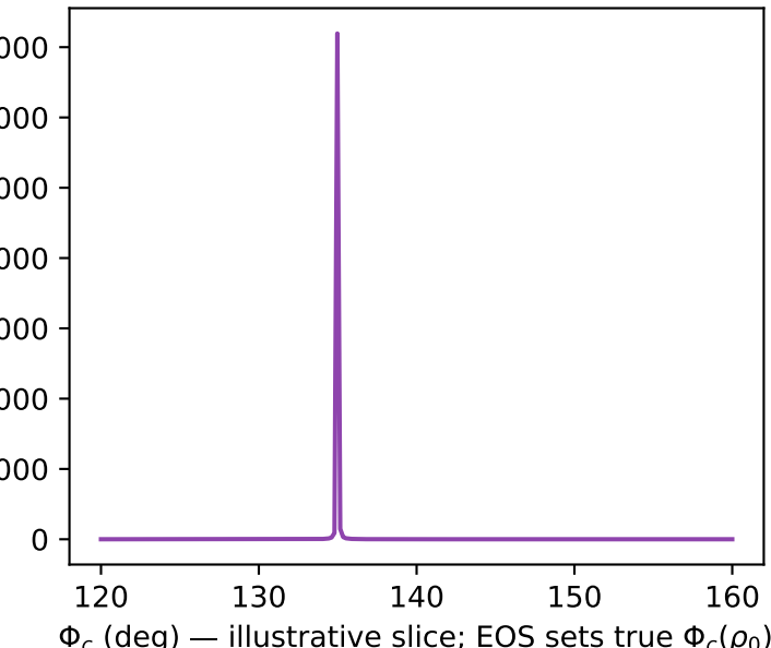
(b) Dimensionless coupling vs chirality slice
