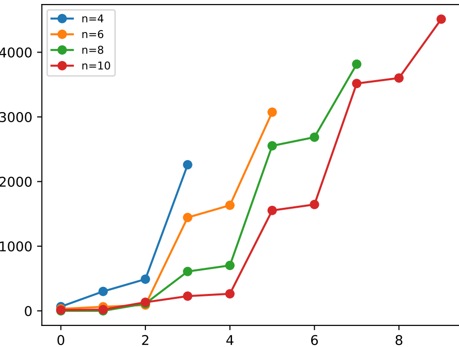
even-n spectra
