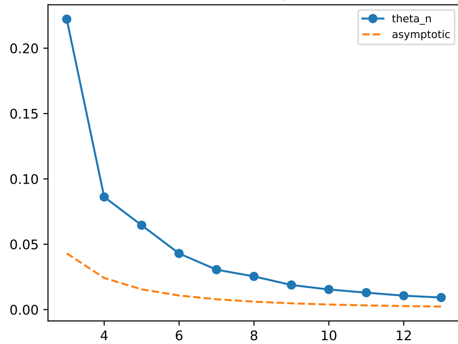
theta convergence
