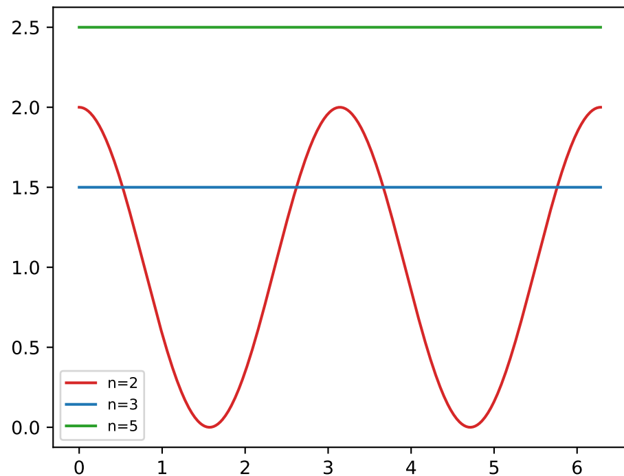
theta convergence
