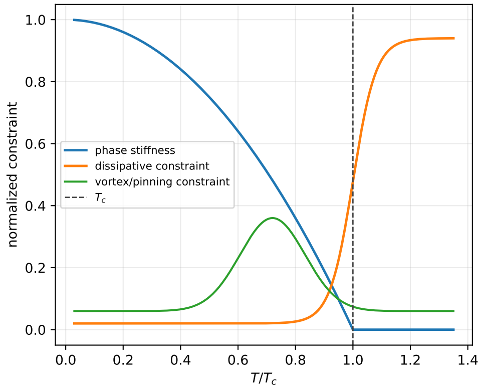
Constraint reallocation
