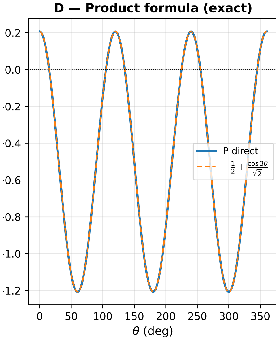
Figure 4: The product formula P(\theta) plotted exactly against numerical evaluation, confirming the closed form representation.
