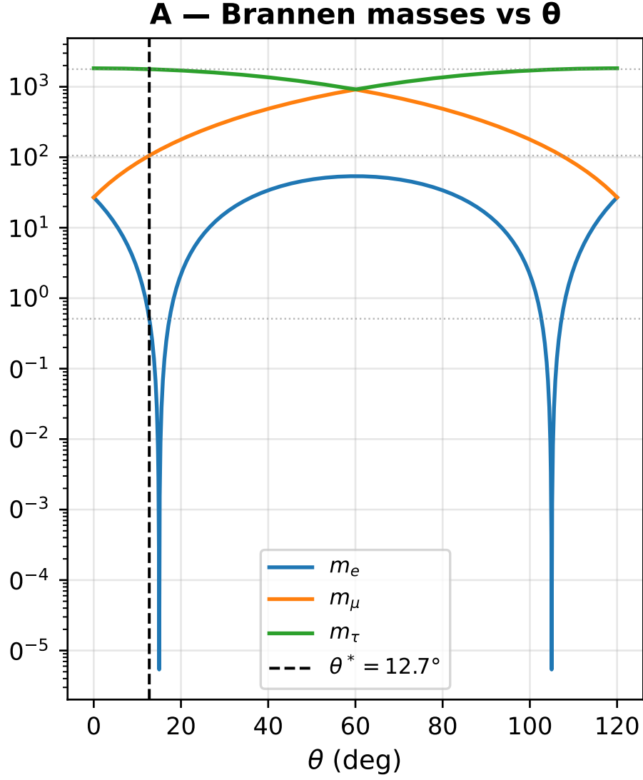
Figure 5: The Brannen masses plotted against \theta . The vertical line indicates the fitted phase \theta^* \approx 12.73^\circ which simultaneously crosses all three PDG mass values (horizontal dashed lines).
