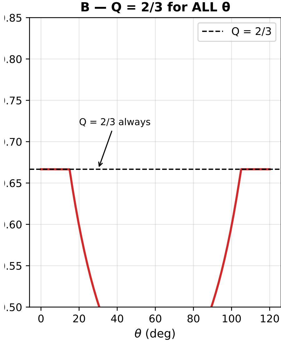
Figure 3: The Koide ratio Q evaluates to exactly 2/3 for all possible values of \theta , demonstrating that the formula is a direct consequence of the \mathbb{Z}_3 symmetry rather than a parameter-tuned coincidence.
