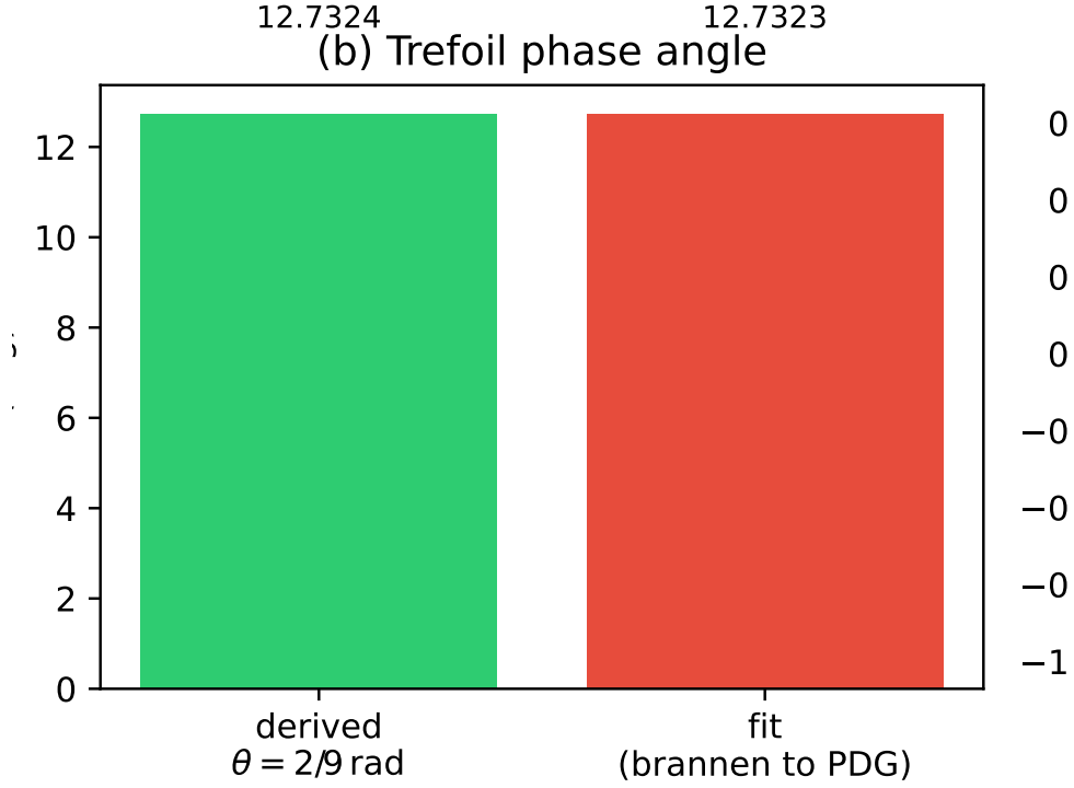
Figure 1: The trefoil phase angle \theta . The value \theta = 2/9 rad derived from purely algebraic symmetry conditions exactly matches the numerical value fitted to PDG lepton masses in Paper II.
