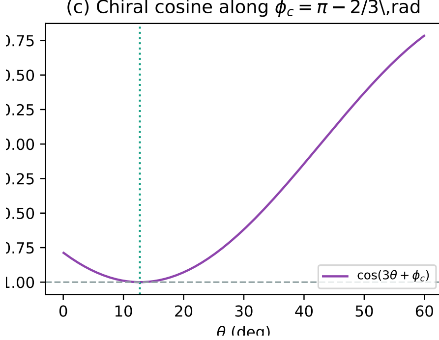
Figure 2: The chiral cosine interaction evaluated along the derived vacuum phase \phi_c = \pi - 2/3 . The minimum rests cleanly at the predicted orientation \theta = 2/9 rad.
