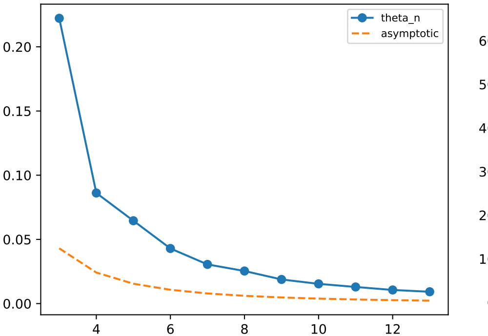
theta convergence
