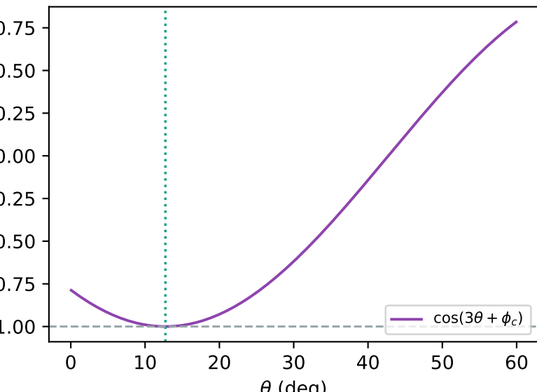
(c) Chiral cosine along \phi_c = \pi - 2/3 \backslash, \text{rad}
