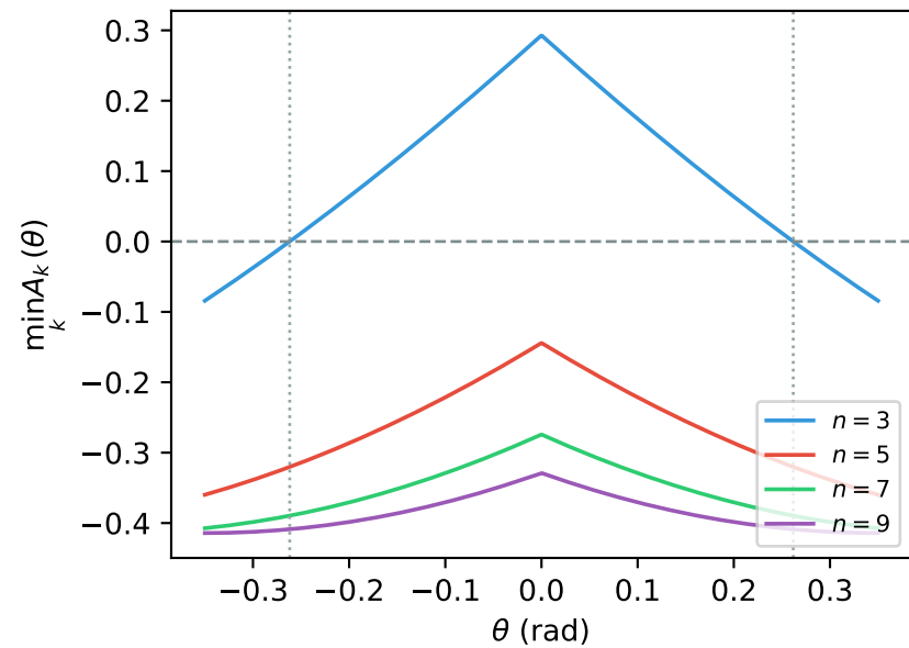
(a) Brannen amplitudes: c_n = \sqrt{2}
