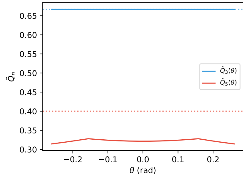
(c) Modified ratio \sum A_k^2 / (\sum |A_k|)^2
