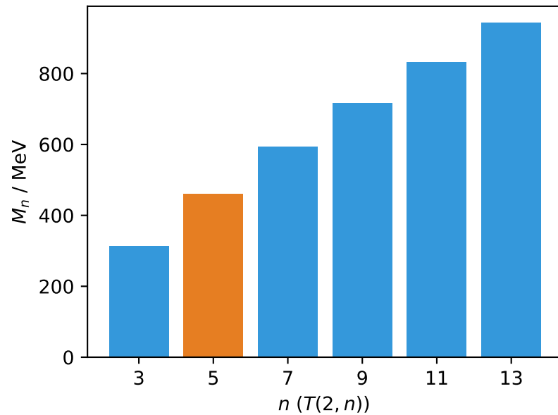
(b) M_n = M_3(n/3)^{3/4}
