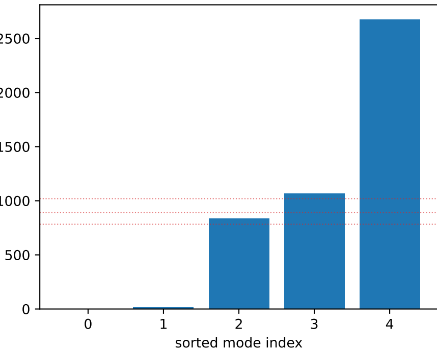
\mathbb{Z}_5 spectrum (PDG refs in table)
