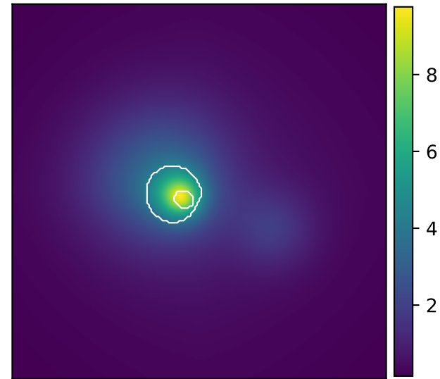
ratio \Psi_p
