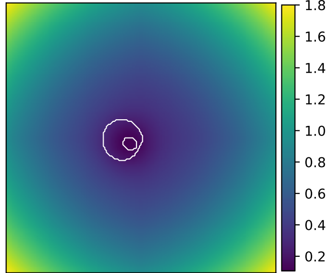
constraint C_p
