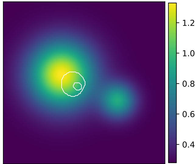
drive \Phi_p
