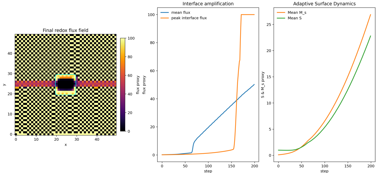
Figure 1: Toy Fe–S interface diagnostic. The left panel shows the final redox-flux proxy with the mineral boundary overlaid; the right panel shows mean flux and peak interface flux across the run. The figure is an illustration of localization under a constraint gradient, not a molecular simulation.
