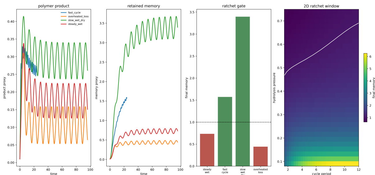
Figure 1: Wet–dry polymerization–ratchet diagnostic. The diagnostic separates product formation from retained memory across several cycling regimes and adds a two-dimensional period–hydrolysis response surface. The model supports a conditional ratchet claim: activation, concentration, retention, and survival must align over repeated cycles.
