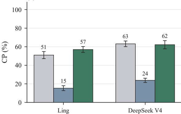
(a) Execution-valid CP
