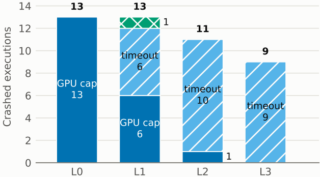
Harness-caused crashes (46 total)
