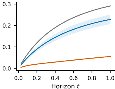
(a) Survival RMSE
