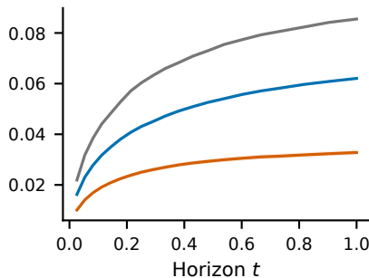
(c) Mean interval width
