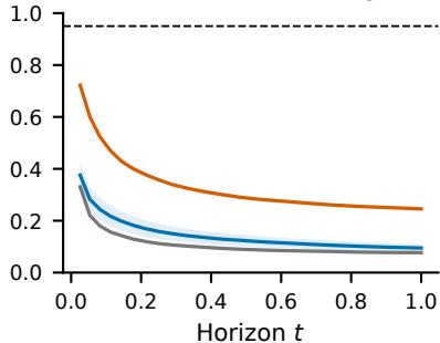
(b) Pointwise 95% coverage
