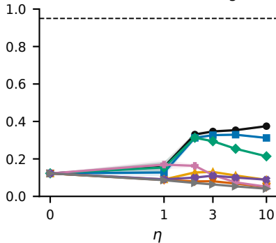
(b) Pointwise 95% coverage
