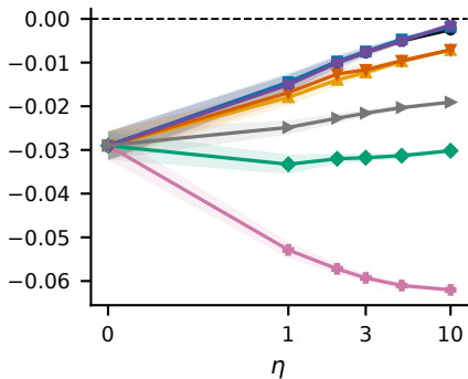
(a) Mean signed error
