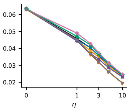
(c) Mean interval width
