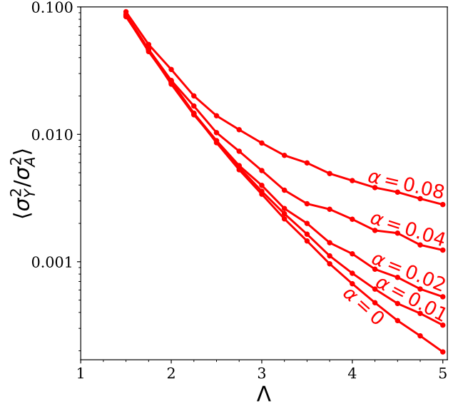
Figure 3.2: The expected accuracy of the emulator falls rapidly with the convergence parameter \Lambda . For this illustration N_{\text{pars}} = 6 and the number of training points was set to 28, the number of expansion coefficients of order n = 2 or less. Calculations were repeated for different values of the point-by-point noise, \alpha . As expected, the impact of the point-by-point noise sets in as the accuracy of the emulator improves.
