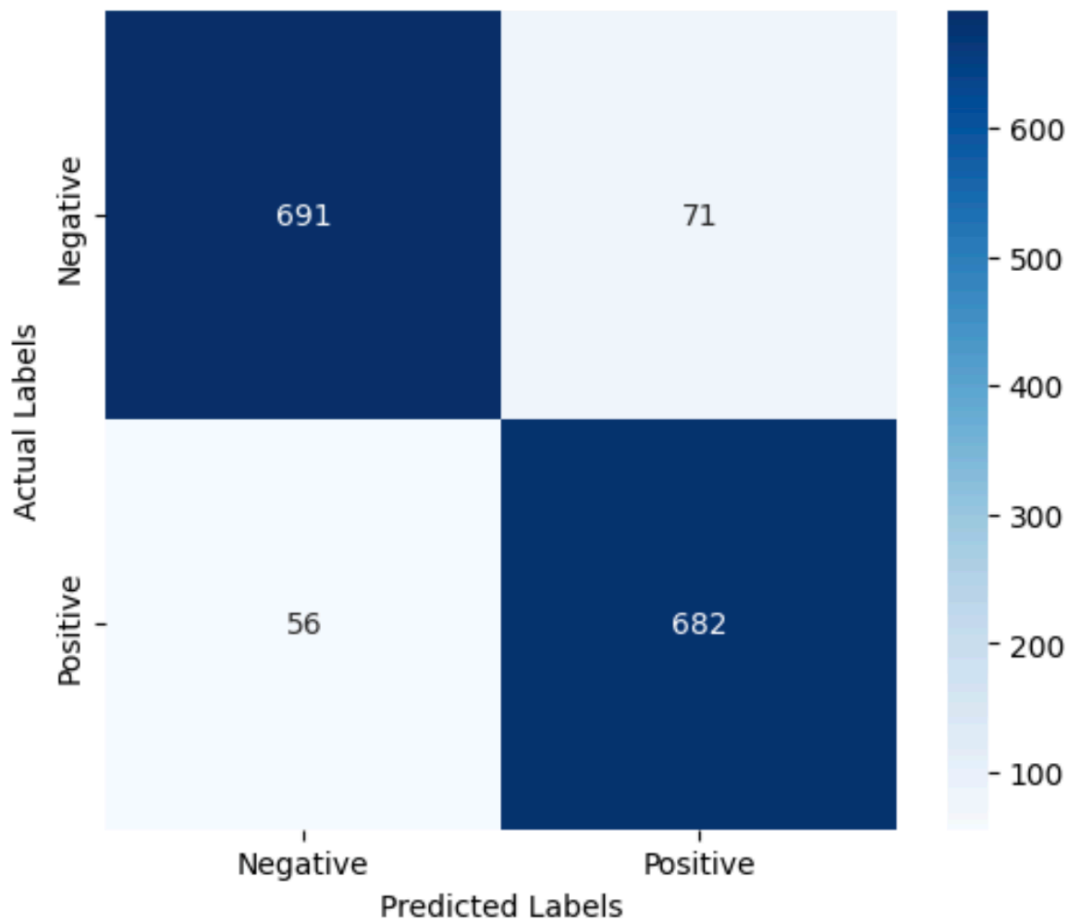
Confusion Matrix
