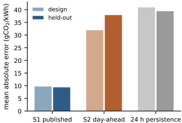
(a) Forecast accuracy
