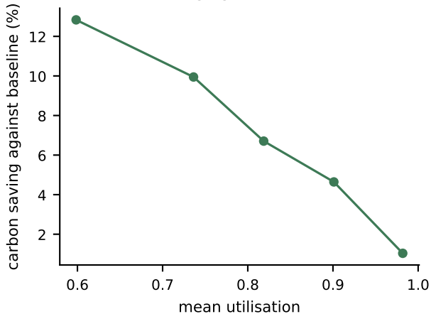
(b) Saving against headroom
