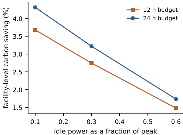
(a) Saving against energy proportionality
