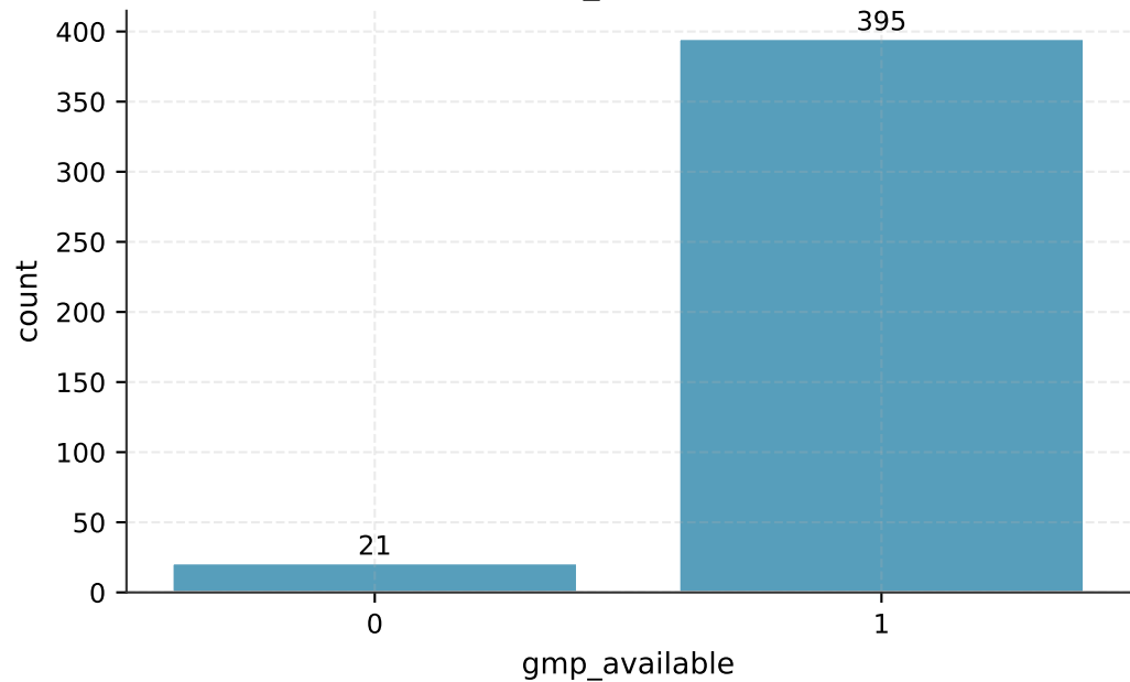
gmp_available
