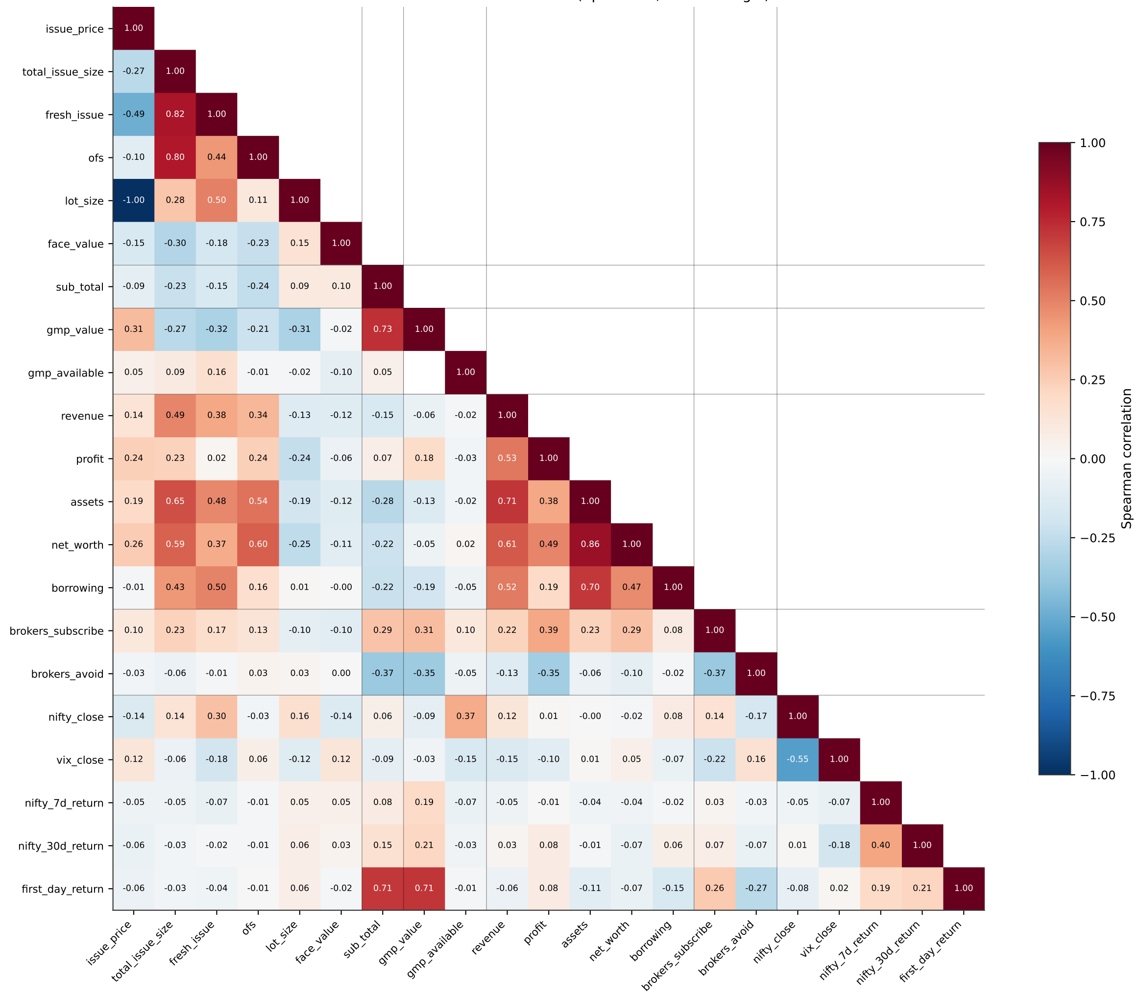
Feature-feature correlation matrix (Spearman, lower triangle)
