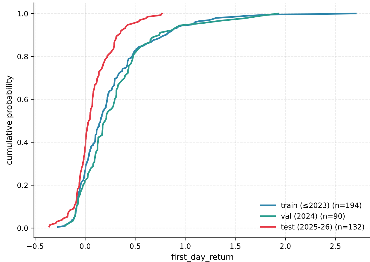
(a) Target distribution — ECDF by split
