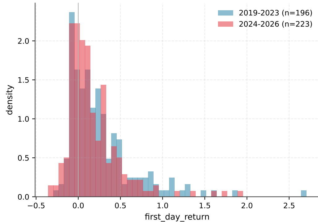
(a) Distributions by regime (Mann-Whitney p=2.85e-02 )
