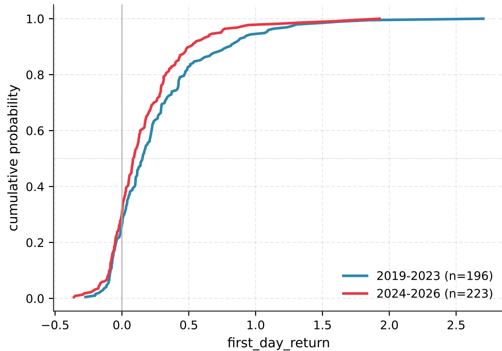
(b) ECDF by regime
