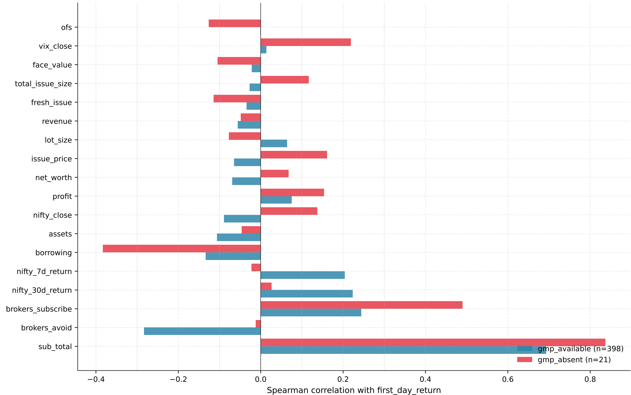
Feature-target correlations by GMP availability subset
