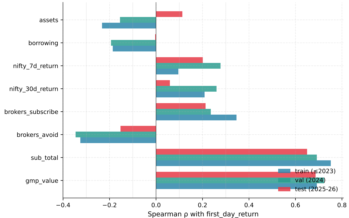
(b) Feature-target correlations by split
