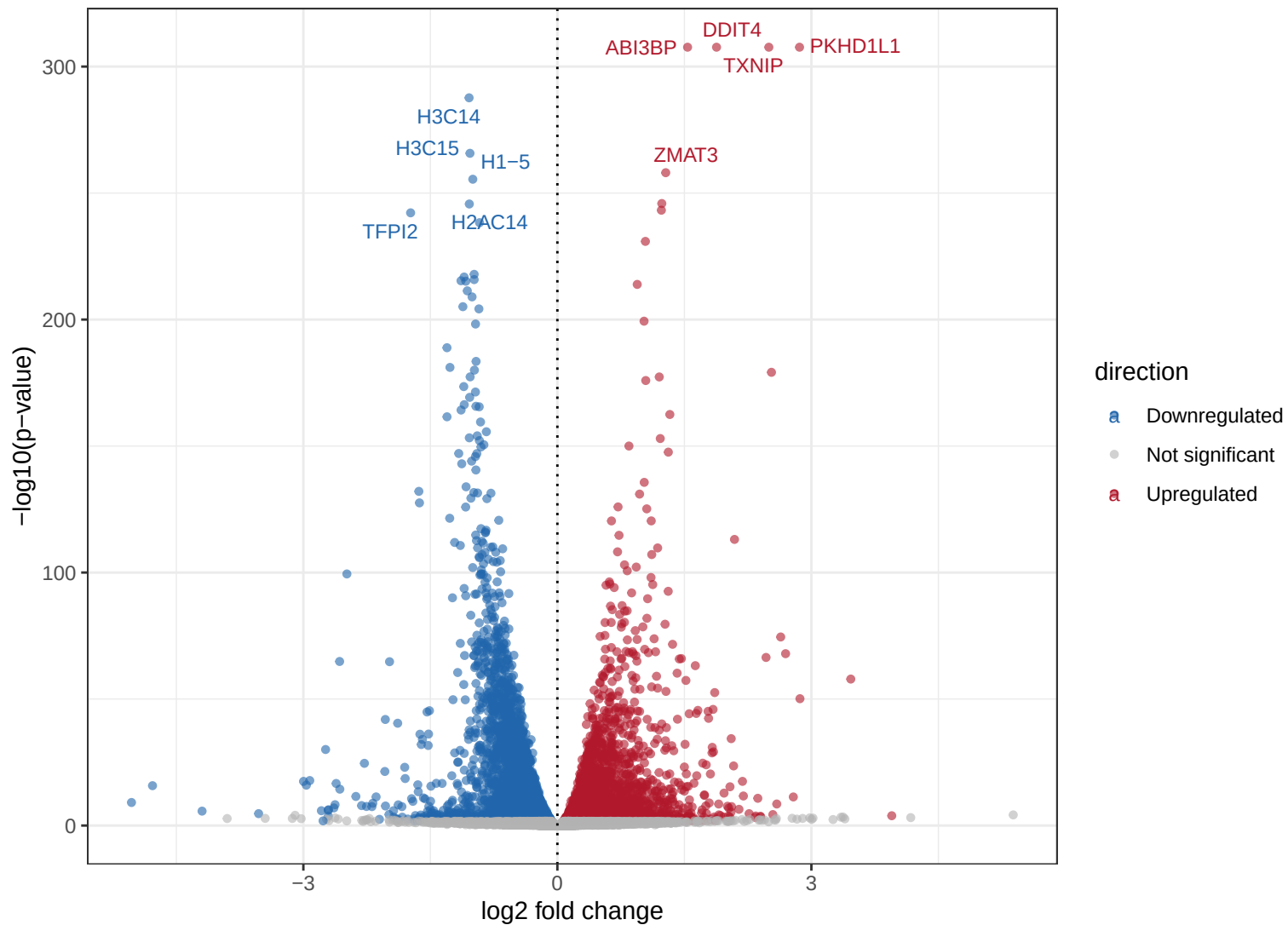
Comparison 2: HUVEC_IR Senescent vs Control
