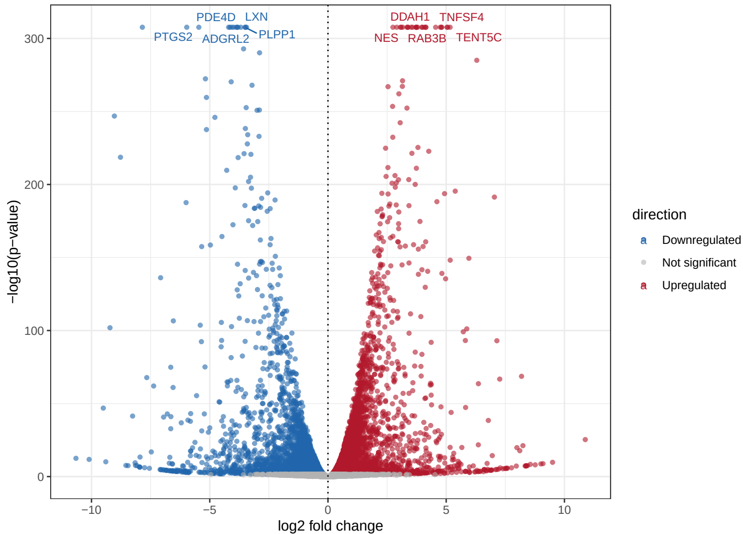
Comparison 4: IMR90_RE Senescent vs Control
