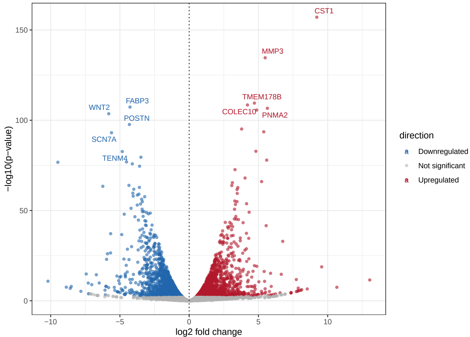
Comparison 8: WI38_RE Senescent vs Control
