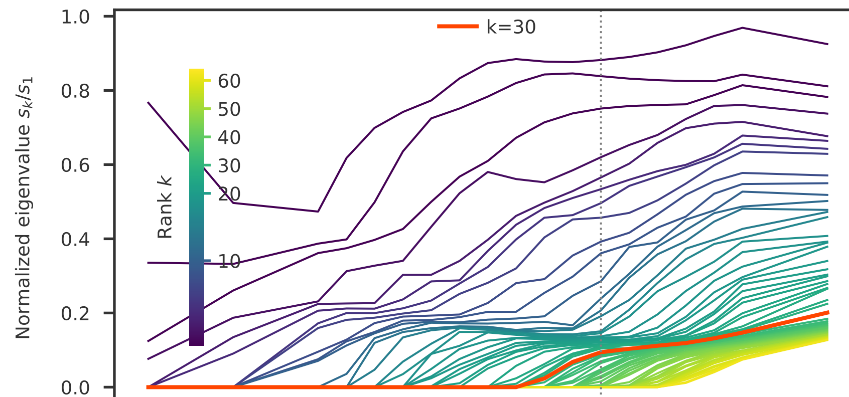
NNM-Corr / PGD+FW
