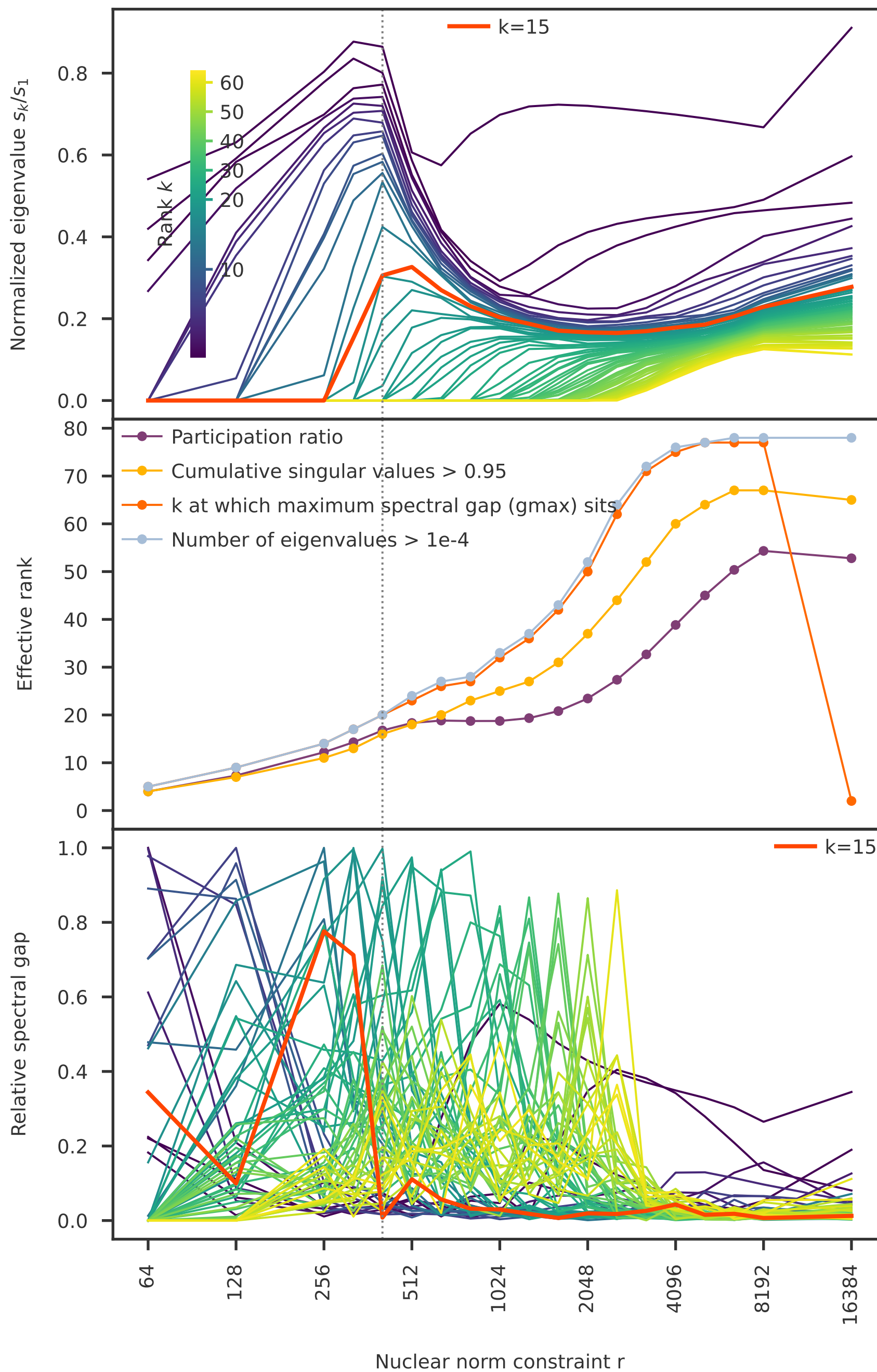
NNM-Corr / PGD+FW
