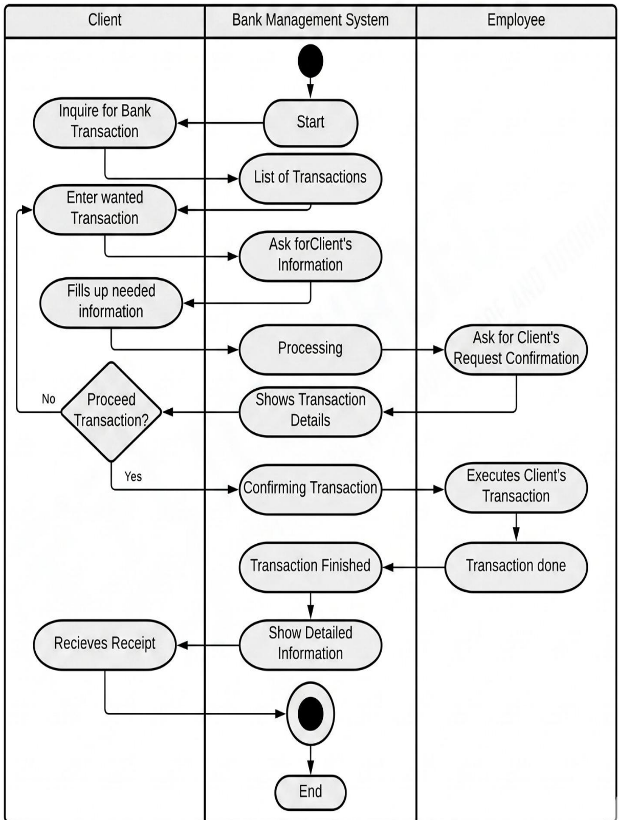
ACTIVITY DIAGRAM
