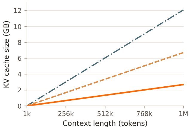
KV cache size
