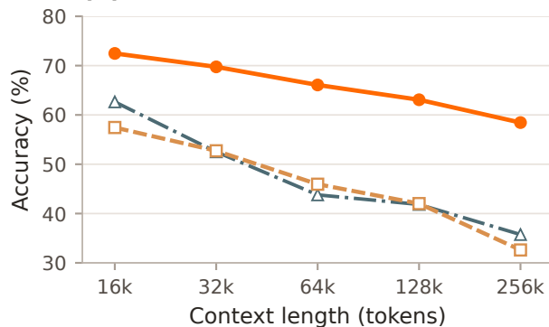
(b) RULER-v2 ↑
