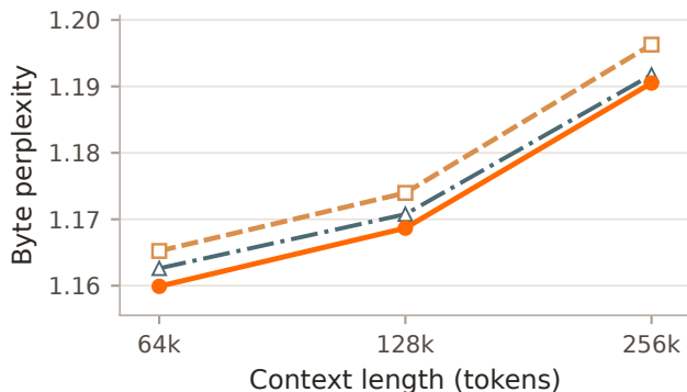
(c) AgentPPL ↓
