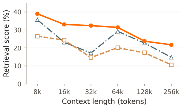
(a) MRCR-v2 ↑
