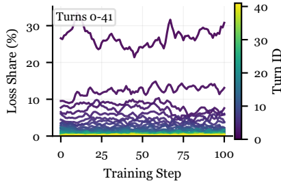
ALFWorld-4B Loss Share
