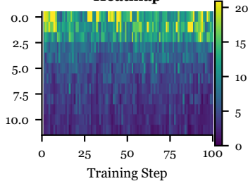
Multi-Hop Search Heatmap
