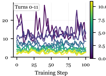
Multi-Hop Search Loss Share
