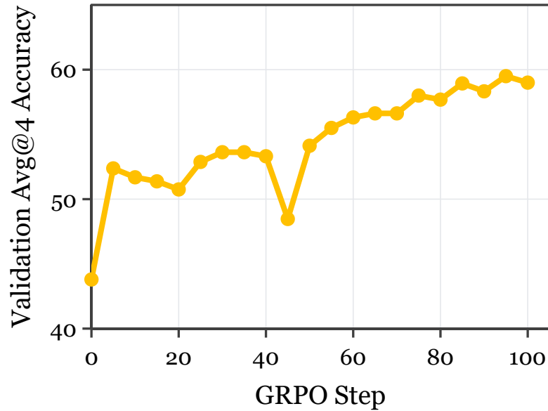
Multi-Hop Search
