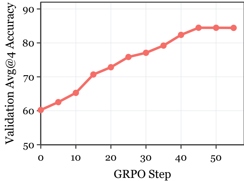
WebShop
