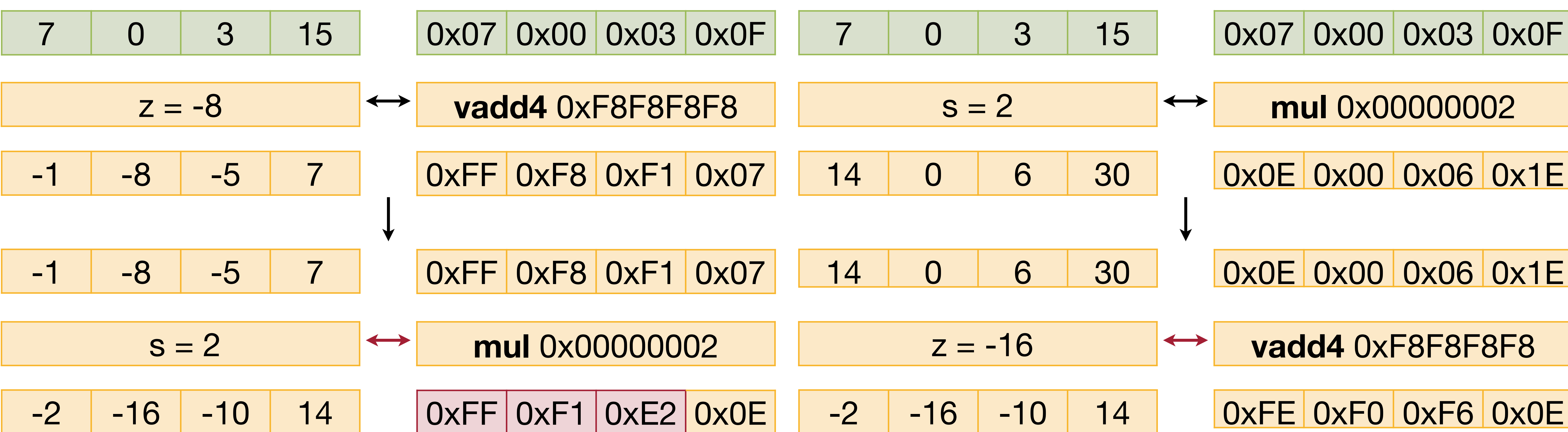
Subtraction before multiplication (a) Overflow fails register level parallelism
