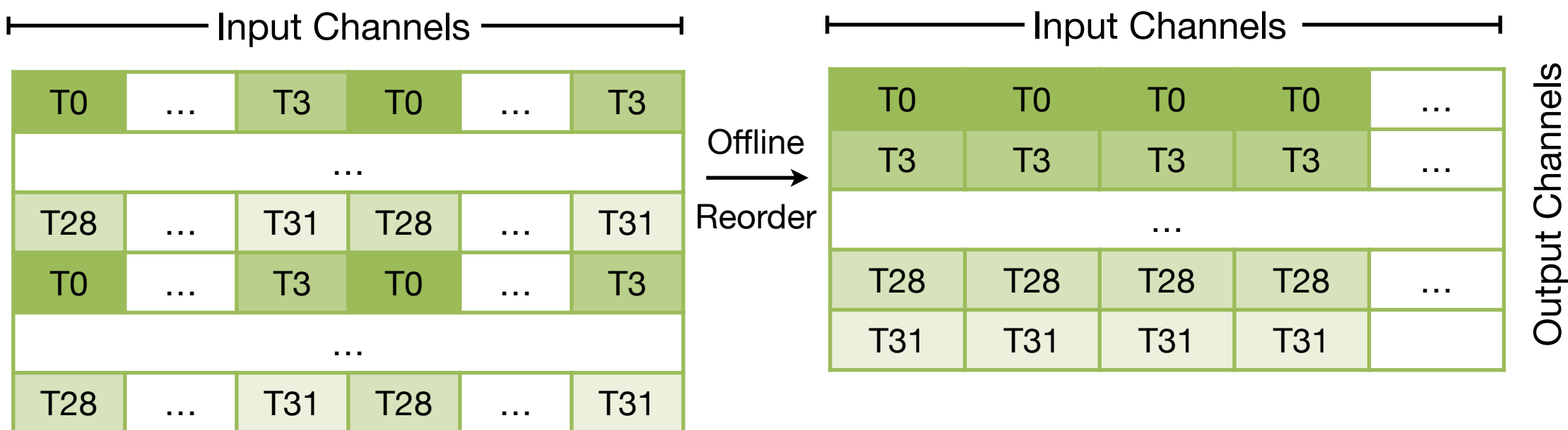
(c) Our solution: compute-aware weight reorder
