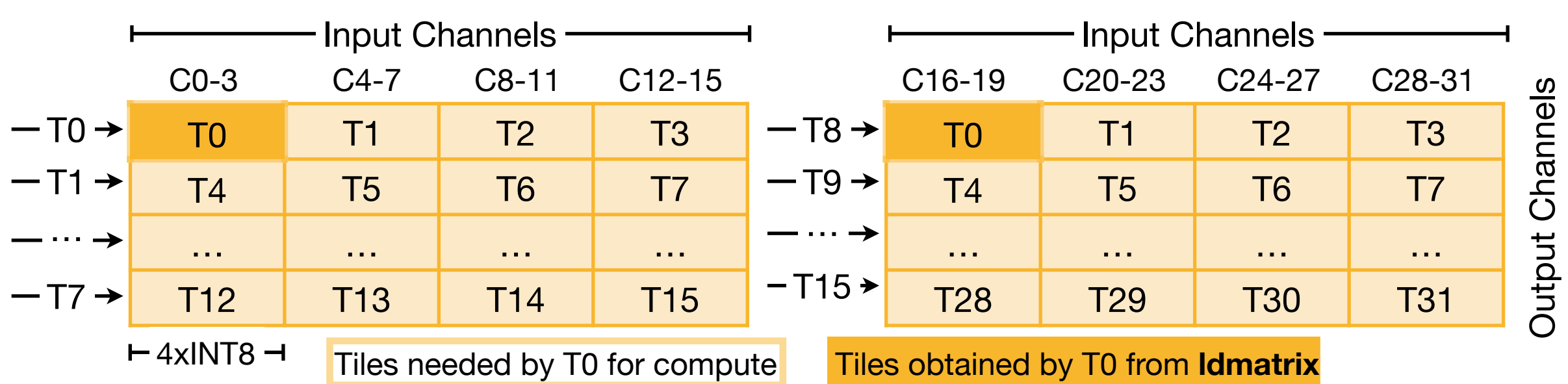
(a) The Idmatrix instruction ensures that each thread gets what it needs for compute in W8A8 GEMM
