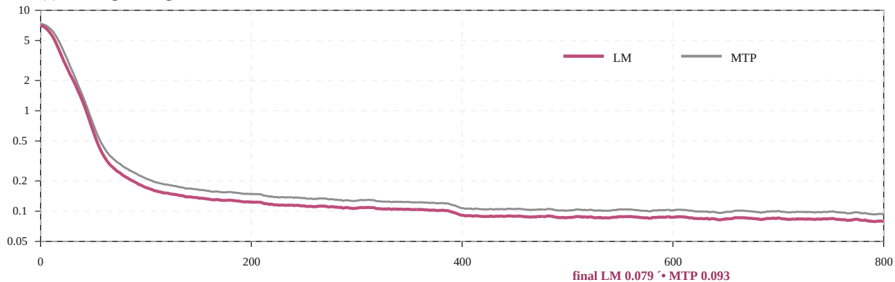
(b) Gradient norm, log scale
