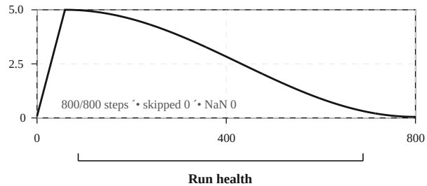
(c) LR schedule ( \times 10^{-6} )
