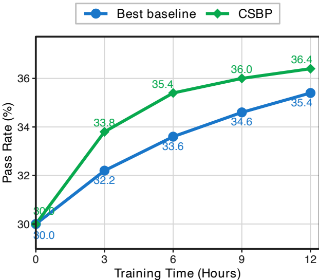
(a) SWE-bench Verified
