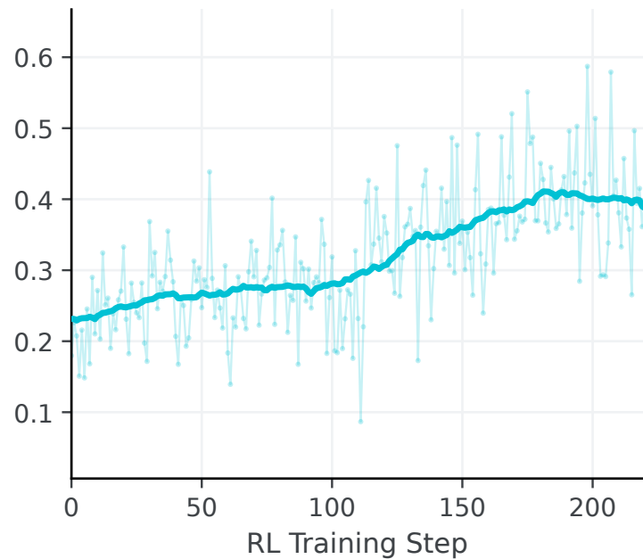
Rollout Base Reward
