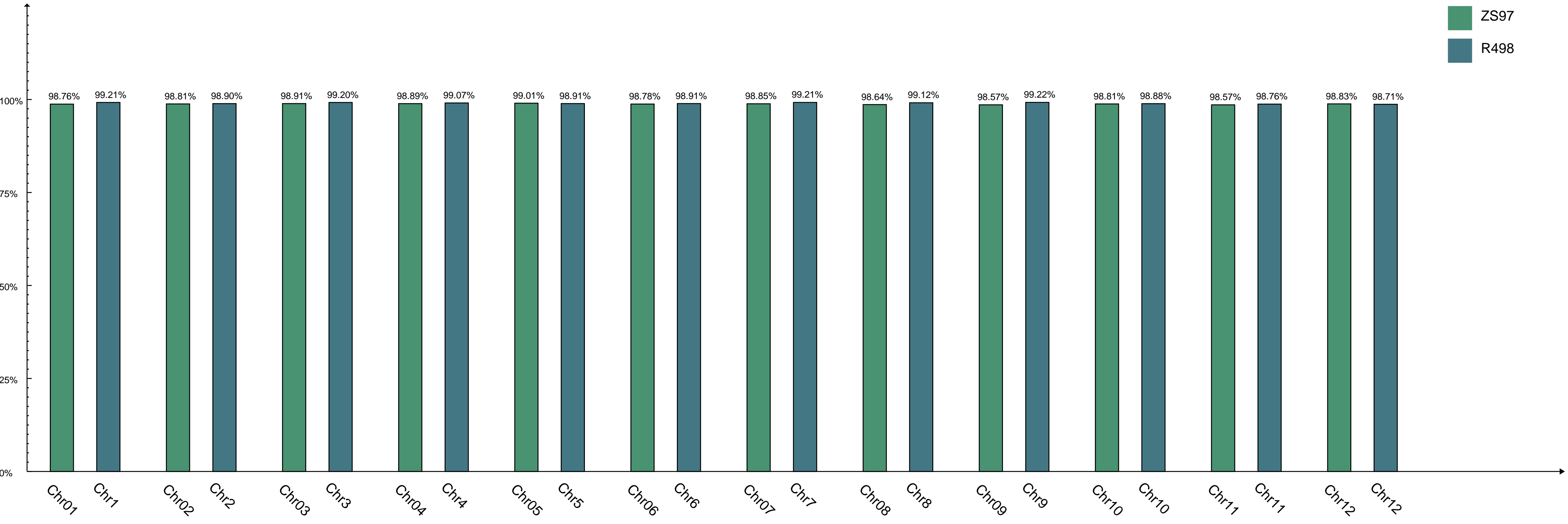
GenomeSyn coverage
